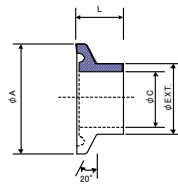
SUS316L #400
